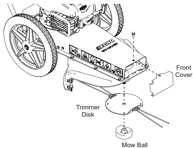
Figure 5.1, Cutting Height Adjustment
